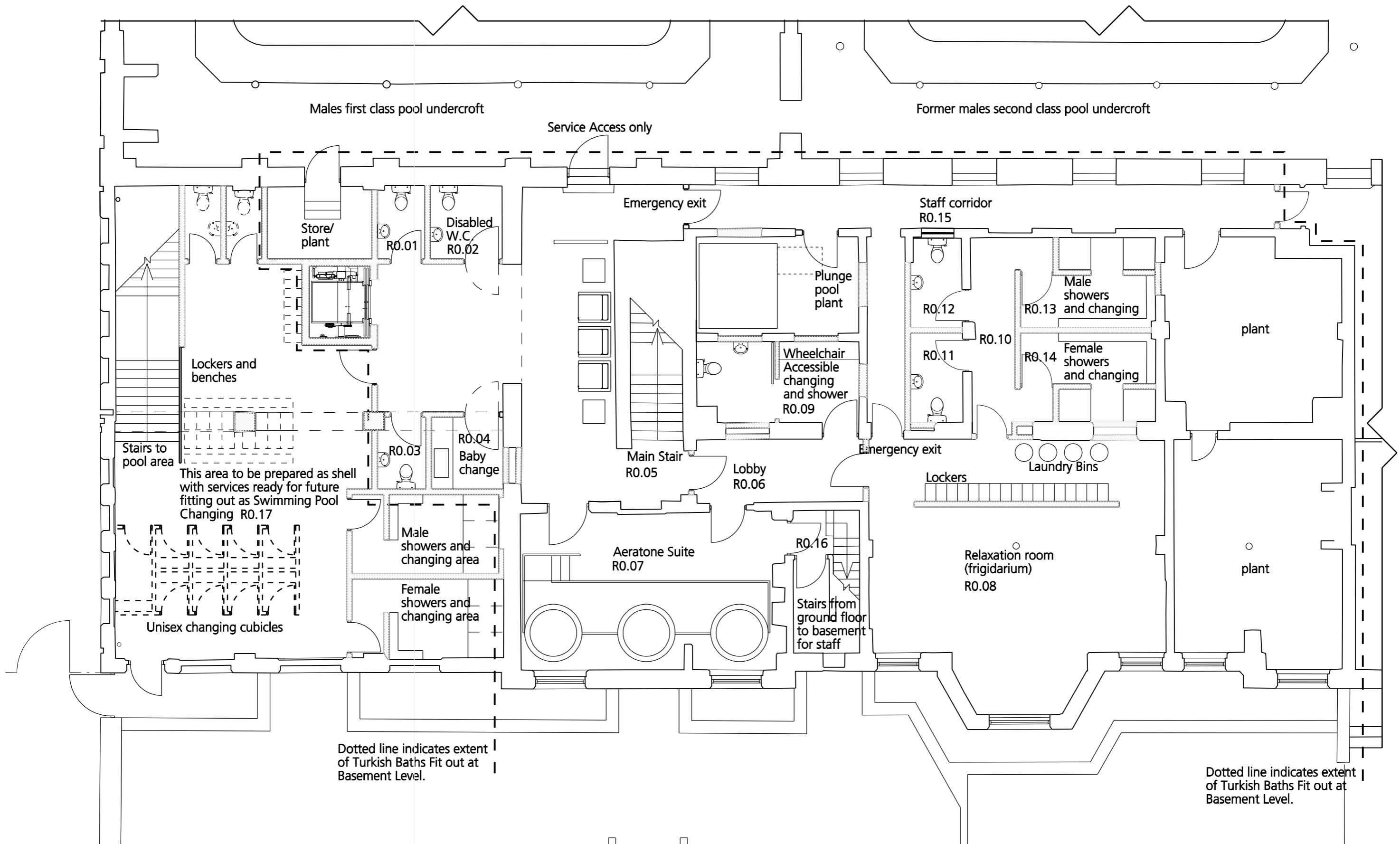
Proposed Basement Floor Plan - Scale 1:100
