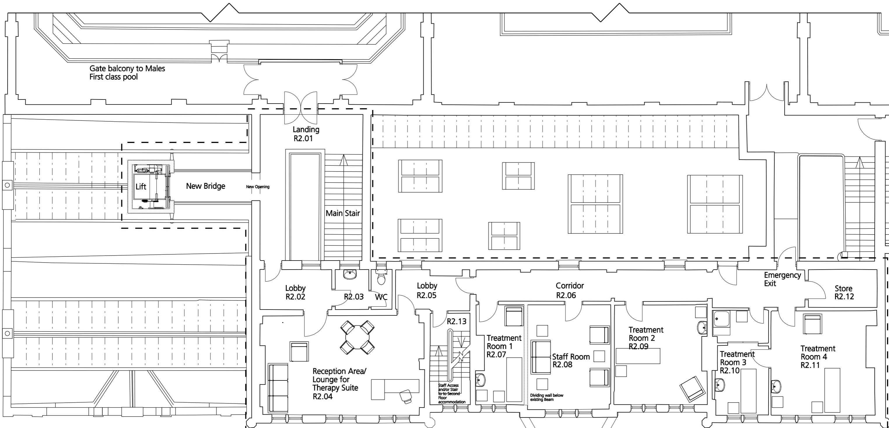
Proposed First Floor Plan - Scale 1:100
